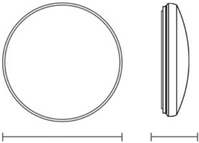
IL-CLSRE360: 360 mm 92 mm
