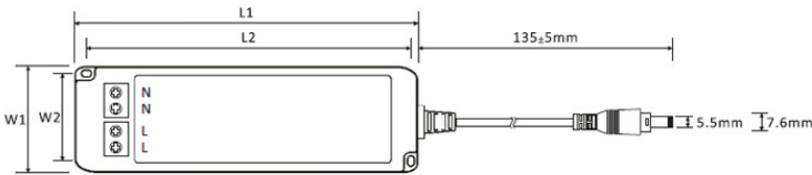
Looping terminals for L and N for easy and quick installation
